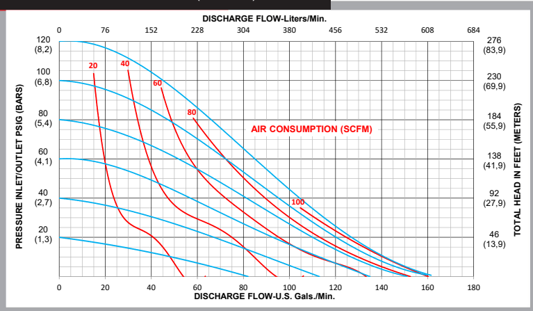
PERFORMANCE CURVE (2" TPE)
