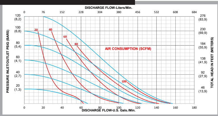
PERFORMANCE CURVE (2" RUBBER)
