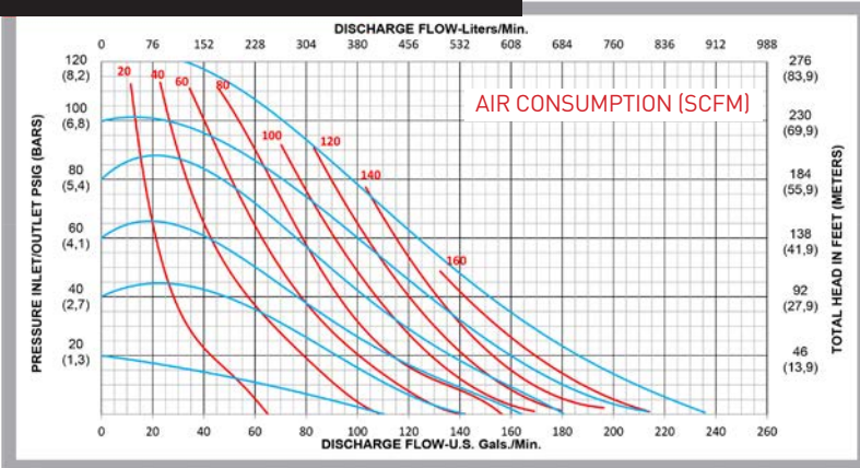
PERFORMANCE CURVE (3" RUBBER)*
