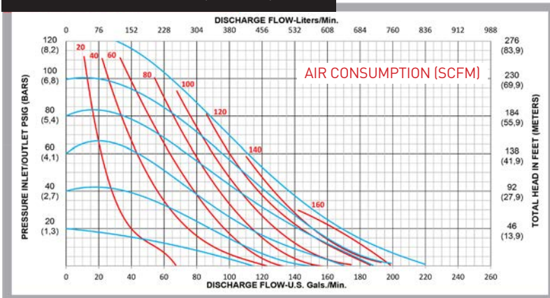
PERFORMANCE CURVE (3" PTFE)*
