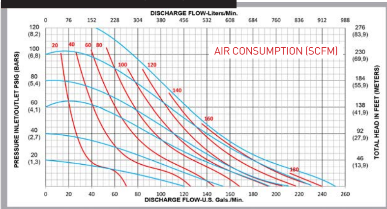
PERFORMANCE CURVE (3" TPE)*
